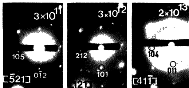
Fig. 2. — Same crystal as in figure 1 during 480 keV Kr ion irradiation. EDP showing different zone axes (see text).
