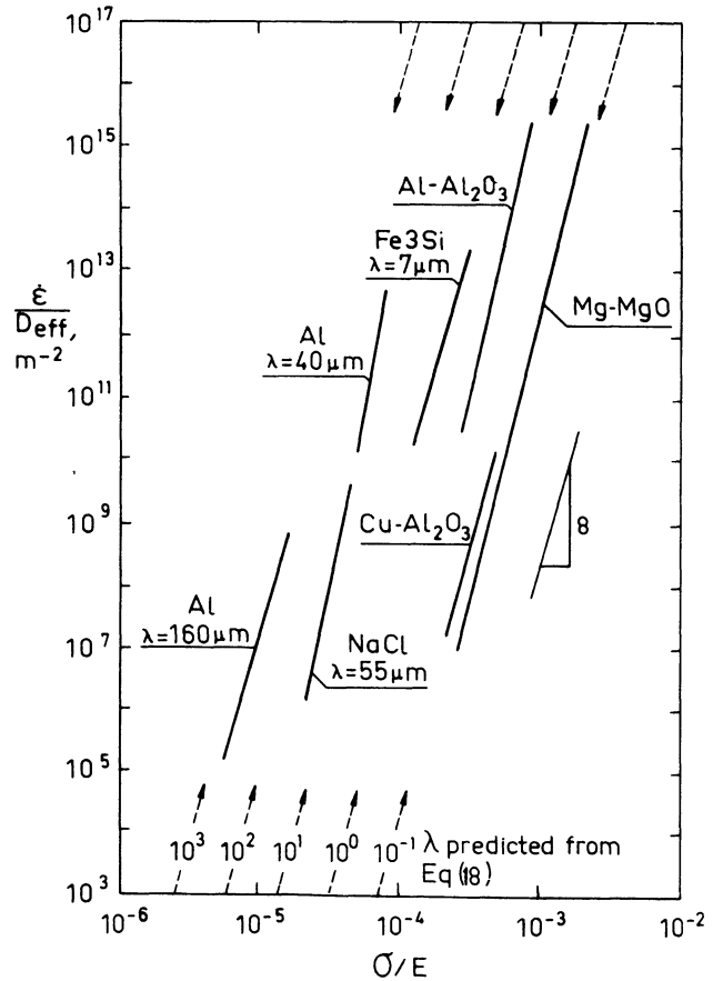
Fig. 6. Diffusion-compensated strain rate as a function of modulus-compensated stress for various materials. Al, Fe-3%Si and NaCl are tested under constant structure conditions.
