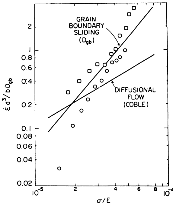
Fig. 9. Comparison of creep data for \beta -Co at 773 (O) and 1073 (□) with predictions from grain boundary sliding ( D_{gb} controlled) and diffusional creep (Coble).
