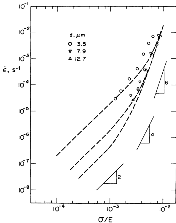
Fig. 5. The steady state creep rate as a function of the modulus-compensated stress for a fine-grained Cu-Al-Si-Co alloy at 500°C. \circ d=3.5 \mu\text{m} ; \nabla d=7.9 \mu\text{m} ; \Delta d=12.7 \mu\text{m} . The broken lines are predicted from Eq. (16) where the pipe diffusion term was neglected.
