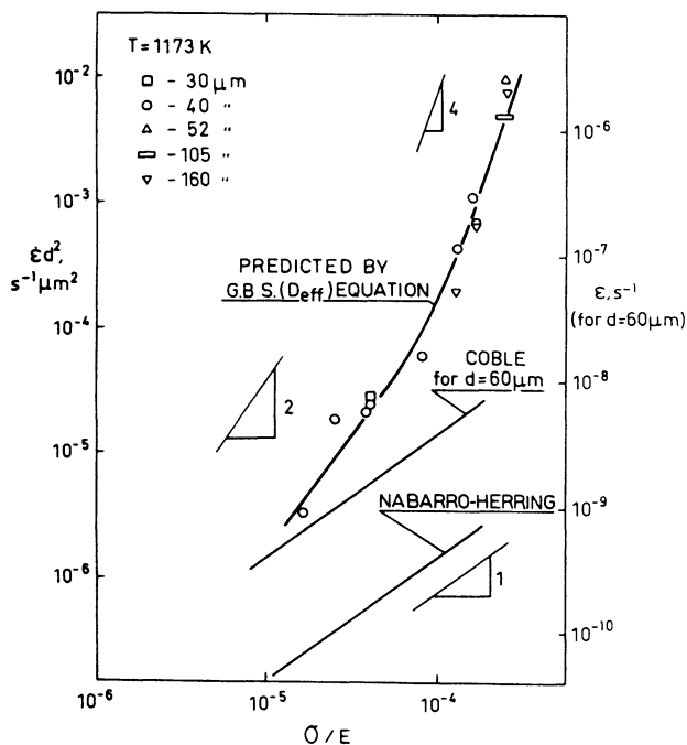
Fig. 11. The predicted grain-size-compensated strain rate-modulus-compensated stress relations for both grain boundary sliding and diffusional creep flow models are shown with experimental data for 25Cr-20Ni stainless steel (from Yamane et al. [91]).
