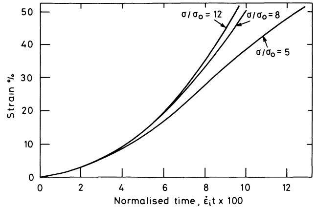
Fig 9: Predicted values of creep strain as a function of \dot{\epsilon}_i t ; derived from Eq's 39 - 41.
