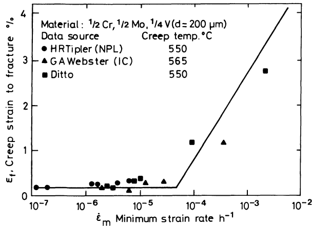
Fig 8: Creep strain at fracture plotted as a function of minimum strain rate for a \frac{1}{2} Cr \frac{1}{2} Mo \frac{1}{4} V steel with a grain size of 200 \mu\text{m} . Two data-sources are used. Creep constrained cavity growth occurs at strain rates below 5 \times 10^{-5} \text{h}^{-1} , while unconstrained growth occurs above that value.
