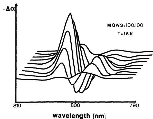
Fig. 4. — Differential absorption coefficient at different time delays (100 fs apart) corresponding to the non resonant excitation (optical Stark effect). The h-h exciton is at 802.5 nm and the l-h at 797 nm.
