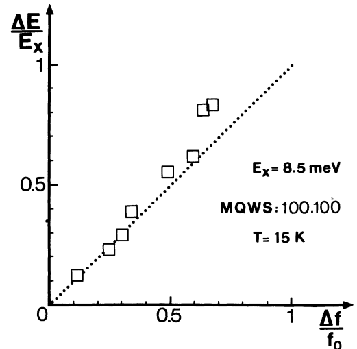
Fig. 5. — Relative h-h exciton energy shift in function of the relative decrease of the oscillator strength.
