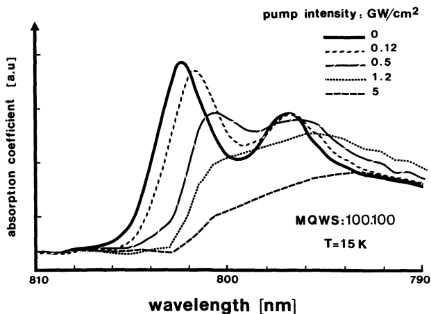
Fig. 3. — Time-resolved absorption spectra of a MQWS at 15 K during the presence of an intense optical pulse at 827 nm for different pump intensities. The wells and the barriers are both of 100 Å width.
