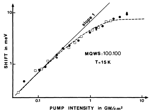
Fig. 6. — Variation of the h-h exciton energy in function of the pump intensity on a log-log scale. The dotted line corresponds to the linear law, the dashed line to expression (8) in the text.
