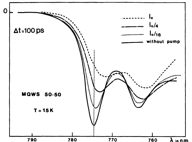
Fig. 2. — Transmittance spectra of a GaAs-AlGaAs MQWS at 15 K in presence of excitons for different pump intensities. The excitons are obtained from the recombination of free carriers (100 ps after their creation).
