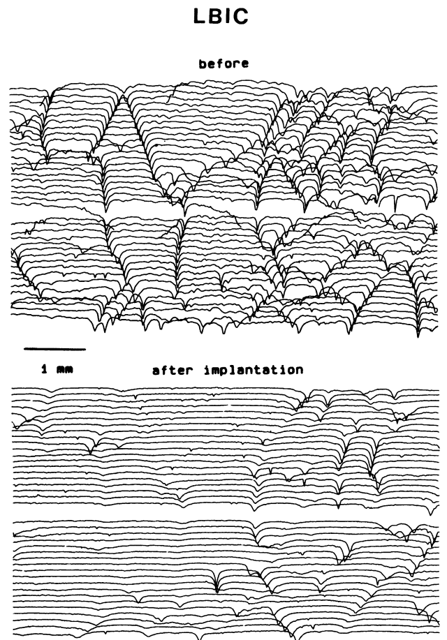
Fig. 6. — LBIC analysis conducted at a wavelength of 0.80 μm on a SILSO cell before and after hydrogen implantation (1 keV, 20 mA, 7 min, temperature ≈ 300 °C).
