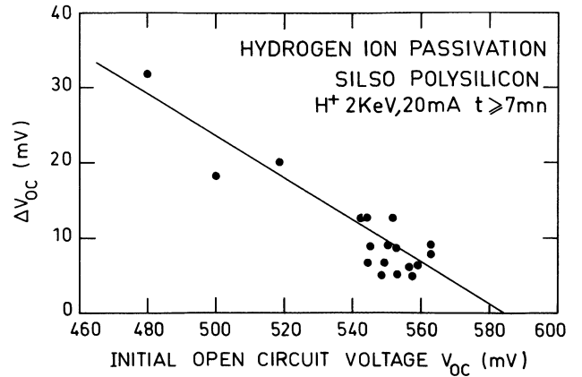
Fig. 5. — Evolution of the enhanced \Delta V_{oc} values vs. the initial open-circuit voltage as obtained on SILSO materials.
