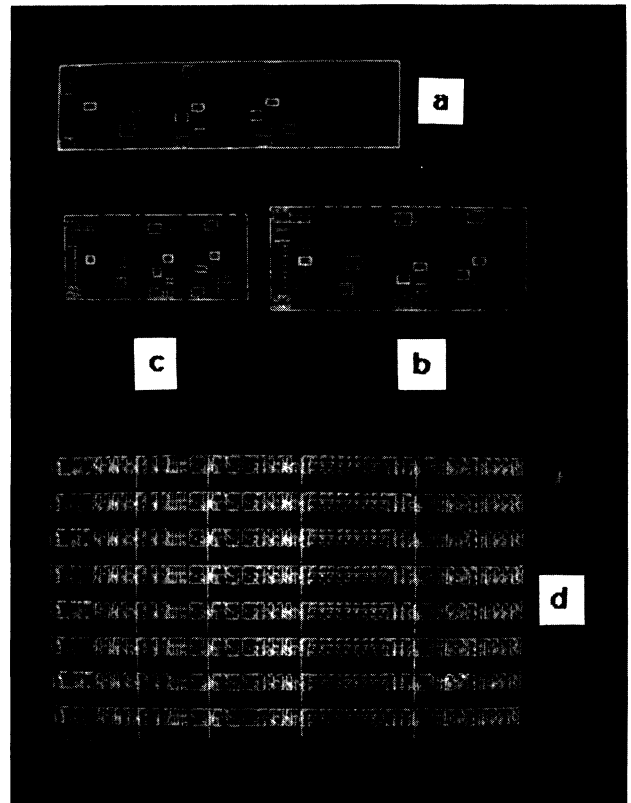
Fig. 9. — a. Symbolically stored cell. b. Spacing for 5\ \mu\text{m} design rules. c. Spacing for 3\ \mu\text{m} design rules. d. Using the cells for composition of 8 bit data path.
