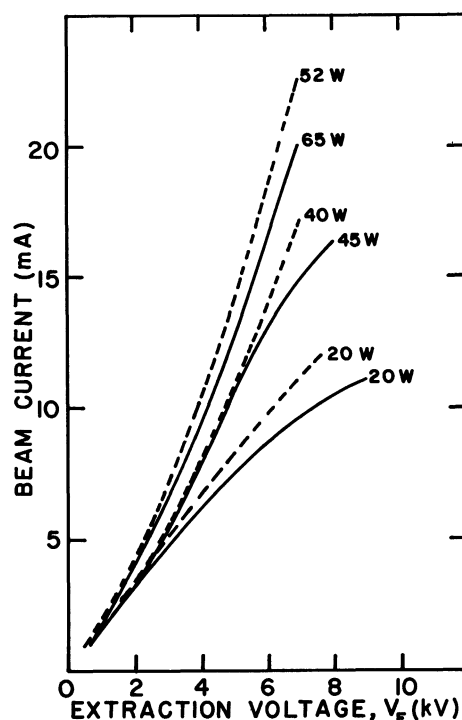
Fig. 27. — Proton beam current yielded by a surface wave based ion source, as a function of the extraction voltage V_E , for various values of the microwave power absorbed by the plasma source. The full lines are from an ion source with a one hole extractor, while the dashed lines correspond to an extractor with seven holes. The hydrogen gas pressure in the plasma source is 0.055 torr for the one hole device and 0.08 torr for the seven hole variant. The surface wave frequency is 870 MHz. The observed ion current dependence on the extraction voltage is within the range V_E^{1.25} and V_E^{1.4} . (From [51].)
