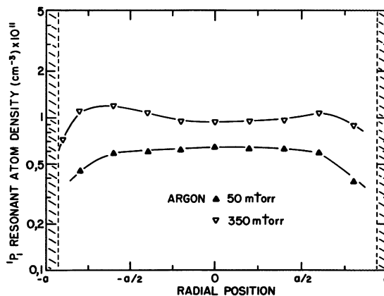
Fig. 18. — Measured density of the ^1\text{P}_1 resonant atoms in argon as a function of radial position in a surface wave produced plasma, for two gas pressures. The wave frequency is 600 MHz and the plasma diameter 26 mm. The density is obtained from optical absorption on the ArI 750.4 nm transition. The plasma column is 200 mm long and the microwave absorbed power is 2 W. (From [21].)
