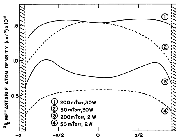
Fig. 19. — Measured density of the ^3\text{P}_2 metastable atoms in argon as a function of radial position, for two gas pressures, when the plasma column completely fills the tube length (200 mm) as a result of multiple reflections of the surface wave on the tube ends (curves 1 and 2). For comparison, the corresponding ^3\text{P}_2 radial density distributions that are obtained when there are no reflections (pure travelling wave) are given as curves 3 and 4. The wave frequency is 600 MHz and the plasma diameter 26 mm.
