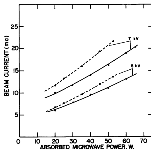
Fig. 28. — Proton beam current yielded by a surface wave based ion source, as a function of the microwave power absorbed by the plasma source. The full lines are from an ion source with a one hole extractor (Fig. 26), while the dashed lines correspond to an extractor with seven holes. Two extraction voltage values are represented, 5 and 7 kV. The hydrogen gas pressure in the plasma source is 0.055 torr for the one hole device and 0.08 torr for the seven hole variant. The surface wave frequency is 870 MHz. (From [51].)
