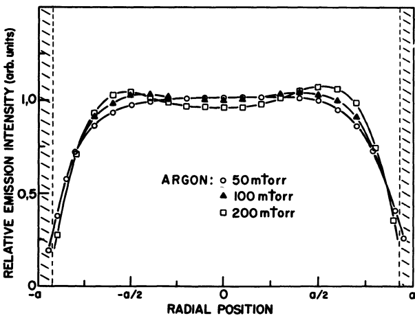
Fig. 12. — Measured relative emission intensity of the ArI 549.6 nm thin line as a function of radial position in a surface wave produced plasma, for three different argon gas pressures. The wave frequency is 300 MHz and the plasma diameter is 26 mm. (From [23].)
