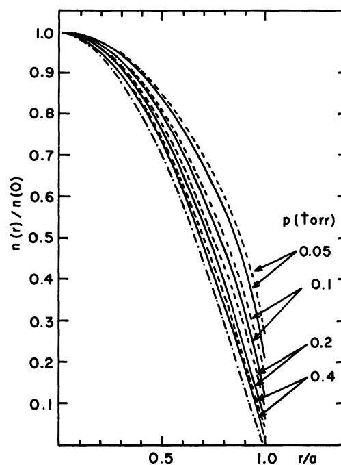
Fig. 5. — Calculated electron density radial profiles in a surface wave produced plasma, for a given average electron density value \langle n \rangle = 10^{11} cm -3 and various argon gas pressures p . The dashed lines are for an isothermal DC positive column plasma of the same diameter, as calculated from the two-moment theory. The dot-dash line is for J_0(2.4 r/a) . The other conditions are those of figure 4.
