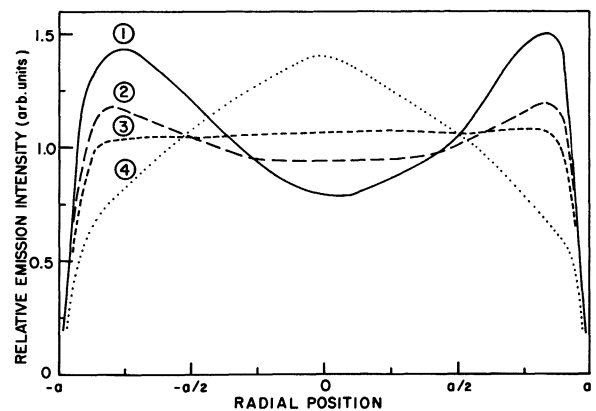
Fig. 16. — Measured relative emission intensity of the ArI 549.6 nm thin line as a function of radial position in a surface or volume wave produced plasma. The gas pressure is 0.2 torr, the plasma diameter is 26 mm, and the wave frequency is 900 MHz. The plasma column is about 1 metre long and it needs about 80 W of microwave power. An axial DC magnetic field can be superimposed on the plasma column : the corresponding electron-cyclotron frequencies f_{ce} are : 0 MHz (1), 950 MHz (2), 1 020 MHz (3), 1 290 MHz (4). At f_{ce} = 0 , the wave is a pure surface wave, while at f_{ce} = 1 290 MHz, it is a pure volume wave. (From [25].)
