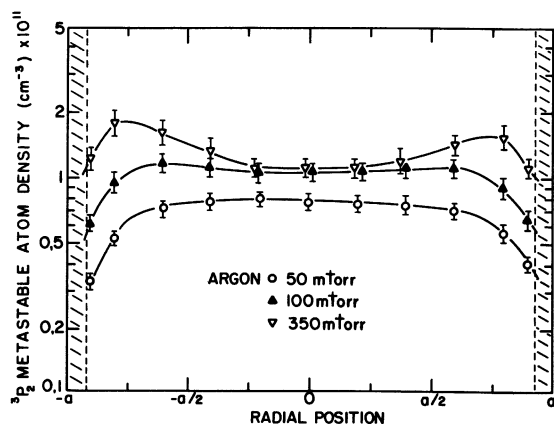
Fig. 17. — Measured density of the ^3\text{P}_2 metastable atoms in argon as a function of radial position in a surface wave produced plasma, for three different gas pressures. The wave frequency is 600 MHz and the plasma diameter is 26 mm. The density is obtained from optical absorption on the ArI 696.5 nm transition. The plasma column is 200 mm long. (From [23].)
