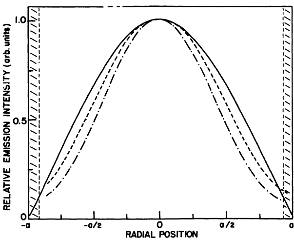
Fig. 11. — Measured relative emission intensity of the ArI 549.6 nm thin line as a function of radial position in the positive column of a DC glow discharge (100 mA), for two argon gas pressures : 0.05 torr (---) and 0.1 torr (-.-.-). The plasma diameter is 26 mm. The full line is given by J_0(2.4 r/a) . (From [23].)
