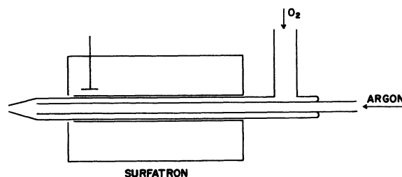
Fig. 30. — Simplified diagram of a general purpose low microwave power plasma source at atmospheric pressures. A surface wave produced argon plasma is generated in the central tube. Then gases (with higher ionization potentials or larger loss rates than argon) are introduced in the outer tube by the lateral inlet. They mix in the nozzle with the excited argon species. This enables one to obtain flames of various compositions. (From [17].)
