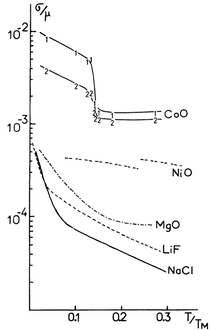
Fig. 6. — Variations with normalized temperature T/T_M of engineering yield stress-shear modulus ratio \sigma/\mu for various NaCl compounds. CoO : T_M = 2\,075 \text{ K} ; NiO : T_M = 2\,235 \text{ K} . MgO : T_M = 3\,098 \text{ K} ; LiF : T_M = 1\,113 \text{ K} ; NaCl : T_M = 1\,074 \text{ K} . For CoO points 1 represent \sigma/\mu_1 and point 2 \sigma/\mu_2 .
