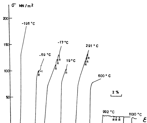
Fig. 2. — Engineering stress-strain curves for CoO single crystals from liquid nitrogen temperature to 1 130 °C. Tests above 600 °C were performed in air. Relaxations are indicated by R and one strain rate change by VC ( 1.5 \times 10^{-5} \text{ s}^{-1} and 6 \times 10^{-5} \text{ s}^{-1} ).
