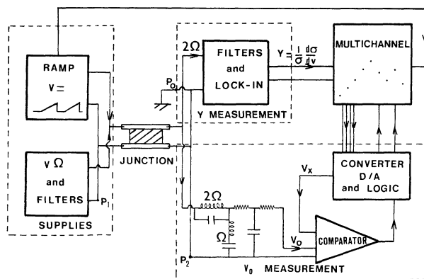
FIG. 8. — Block diagram of circuitry.
