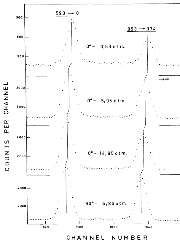
FIG. 1. — Gamma rays from the 593 \rightarrow 0 keV and the 993 \rightarrow 374 keV transitions observed in the ^{40}\text{Ar}(\alpha, n)^{43}\text{Ca} reaction for different gas pressures.
