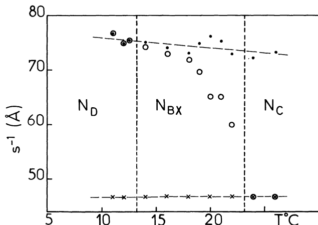
Fig. 3. — Synchrotron X-ray measurements of s_1^{-1} (●), s_2^{-1} (○) and s_3^{-1} (×) as functions of temperature in the three nematic phases. The variations of s_1^{-1} and s_3^{-1} with temperature are visualized by broken lines. The experimental error in the measurements of s_i^{-1} from the microdensitometer profile of the diffraction patterns is about (0.8 Å). The transition temperatures (dashed lines) are determined independently by measuring the optical anisotropies [8].
