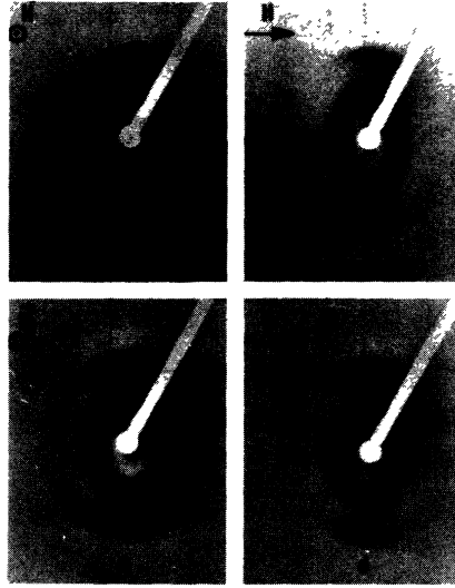
Fig. 1. — Synchrotron X-ray patterns of oriented K-laurate, 1-decanol, D_2O nematic lyomesophases. The capillary is set up in the vertical direction in the plane of the figure. (a) Discotic phase with the director ( \mathbf{n} ) along the vertical direction. T = 12 °C. Note that, for symmetry reasons, the X-ray pattern is the same when \mathbf{H} is in the plane of the figure, perpendicular to \mathbf{n} . (b) Calamitic phase with \mathbf{n} parallel to the magnetic field ( \mathbf{H} ) in the plane of the figure. T = 24 °C. (c) and (d) Biaxial nematic phase with \mathbf{H} parallel and perpendicular to the beam respectively. The sharp band d in figure 2 near the beam stopper more visible in (c) is due to the \lambda/3 radiation. T = 20 °C.
