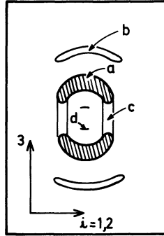
Fig. 2. — Sketch of the diffraction patterns presented in figure 1 with a denomination of the different diffraction bands.
