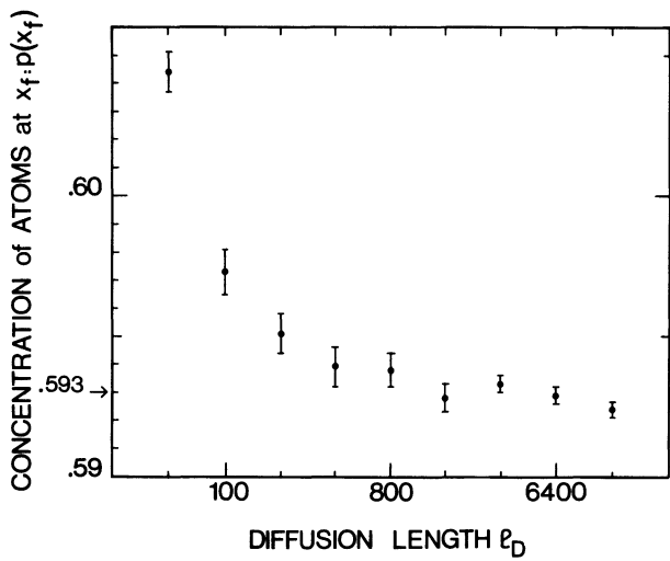
Fig. 5. — Diffused atom concentration at the mean front position x_f as a function of the diffusion length in the case of a square lattice. The approximate value p_c = 0.593 has been represented. The error bars represent statistical uncertainties.
