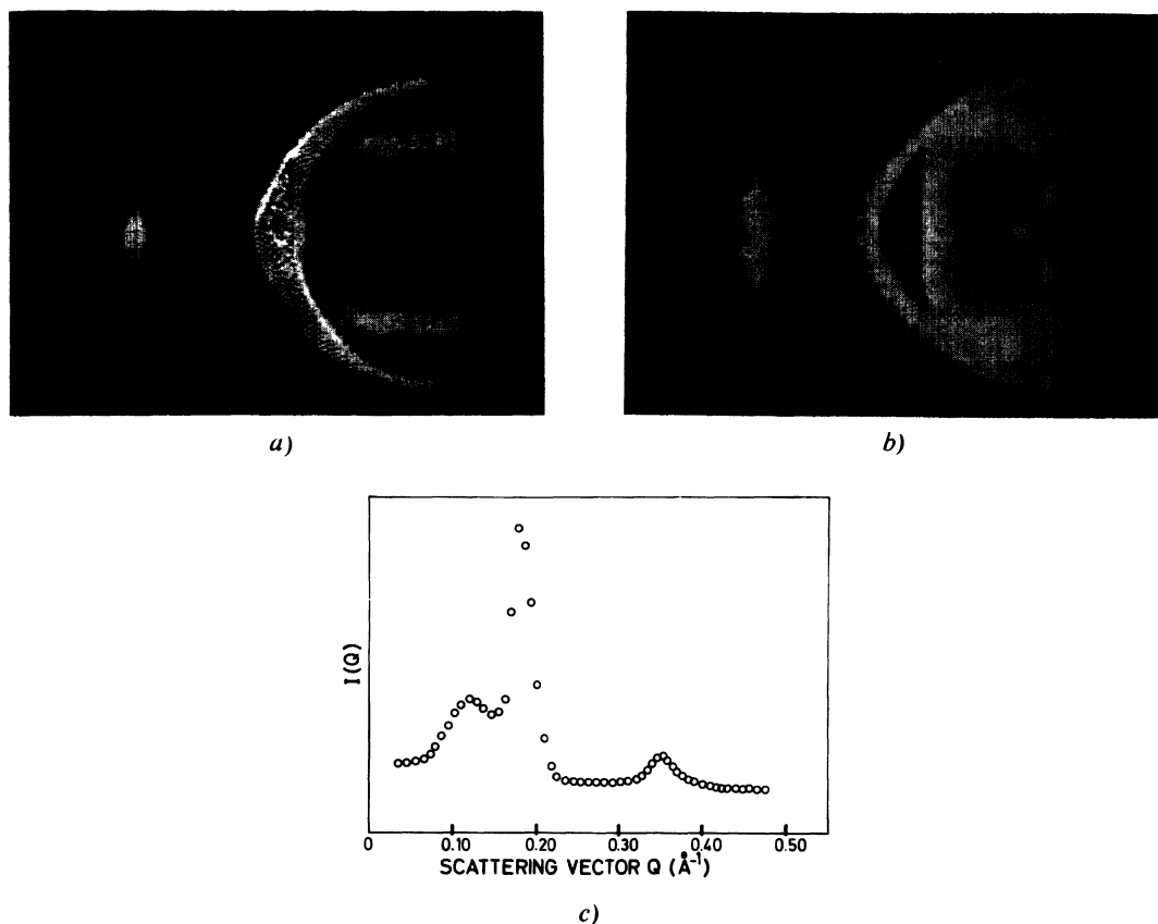
Fig. 3. — (a) A slice at constant intensity of the scattering pattern observed with PAXY; scattering geometry as in Fig. 1(i). The sample is a lamellar phase made of 70.01 % SDS and 29.99 % D_2O at a temperature of 64^\circ C ; it is oriented by a stack of vertical quartz plates. The horizontal axis is the axis of symmetry of the reciprocal space; on this axis are, from right to left, the beam stop, the 1st diffraction order of the layers and the 2nd order. In slices made at lower intensity levels, a cross of diffuse scattering appears around the beam stop. The horizontal stripes are the section of a tube by a radial plane; it is argued that they are caused by diffuse scattering from structural defects in the layers. (b) A slice at a lower intensity level of the same scattering pattern. The cross around the beam is produced by textural defects. (c) Isotropic regrouping of the same scattering pattern; the horizontal stripes give rise to the hump at Q = 0.11 \text{ \AA}^{-1} ; the diffraction orders are at 0.19 \text{ \AA}^{-1} and 0.38 \text{ \AA}^{-1} .
