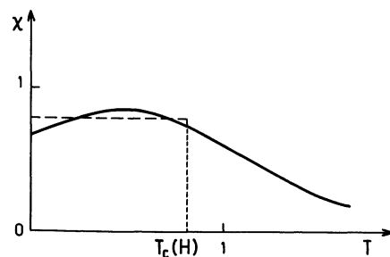
Fig. 3. — The full line represents the magnetic susceptibility \chi_{SK}(T, H) , calculated without replica symmetry breaking, in a small applied field H . The horizontal dashed segment is the prediction of the projection Hypothesis, in the spin glass phase. All three figures are free hand drawings.
