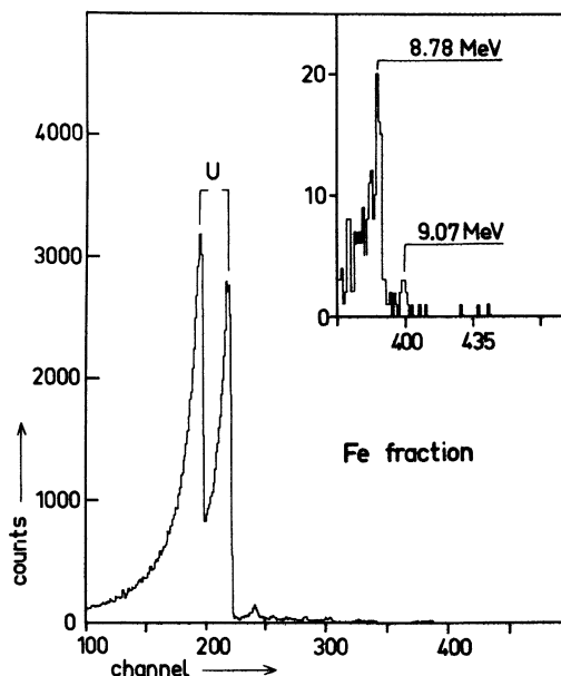
Fig. 3. — Spectrum ( \Delta T = 33 days) showing an unidentified peak at 9.07 MeV.
