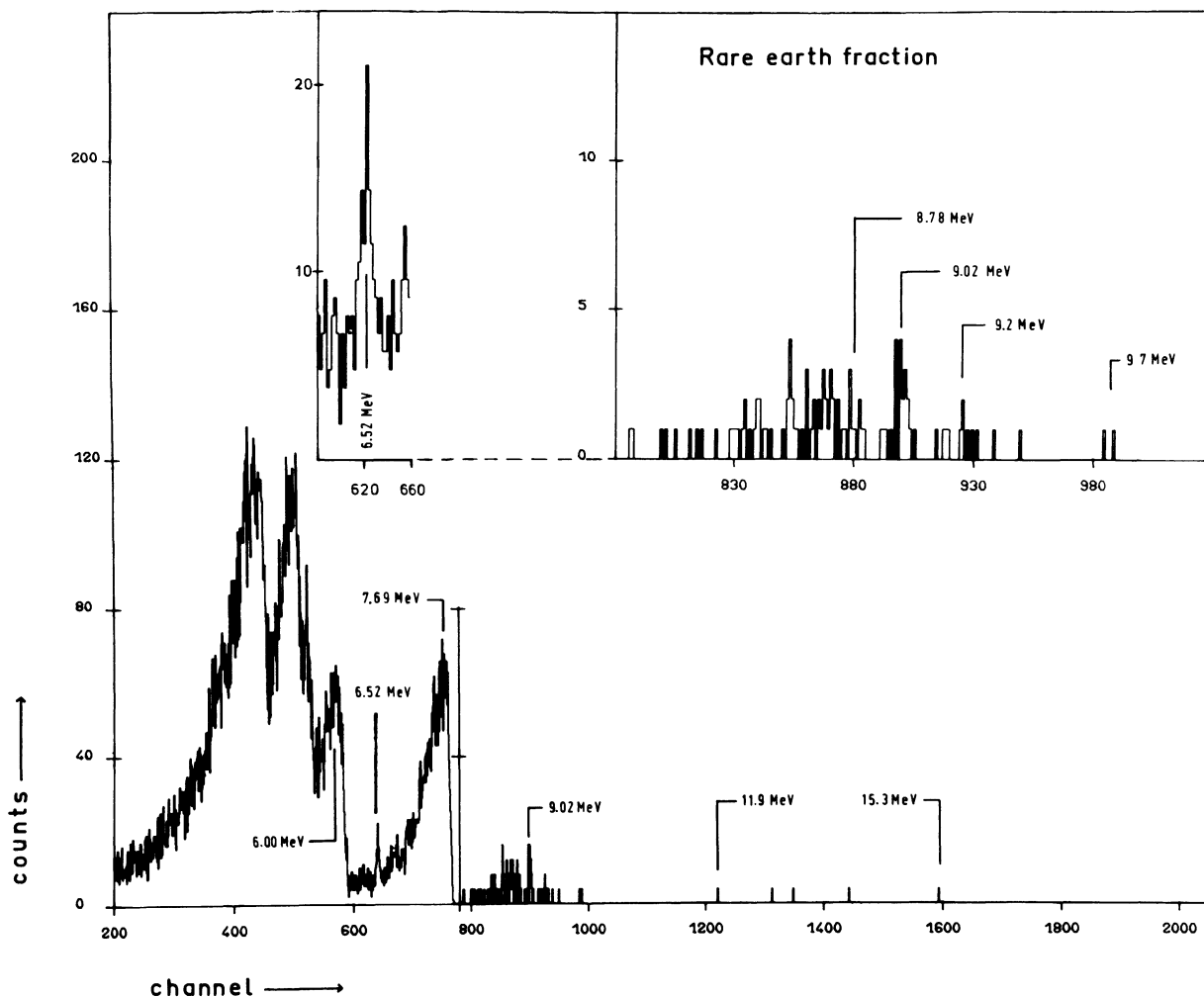
Fig. 1. — Spectrum ( \Delta T = 38 days) showing unidentified peaks at 6.52 and 9.02 MeV, and counts in the 8-10 and 12-15 MeV regions.
