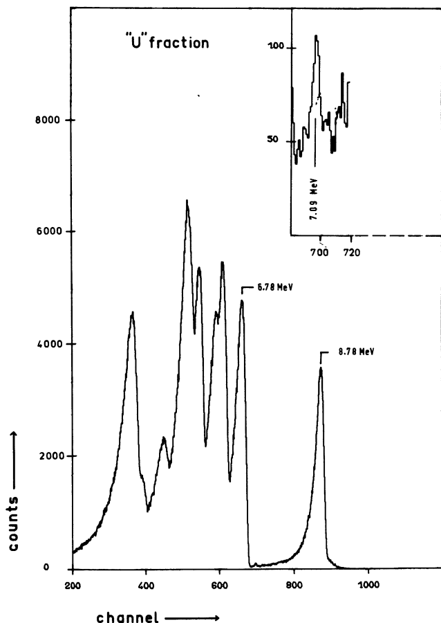
Fig. 2. — Spectrum ( \Delta T = 30 days) showing an unidentified peak at 7.09 MeV.
