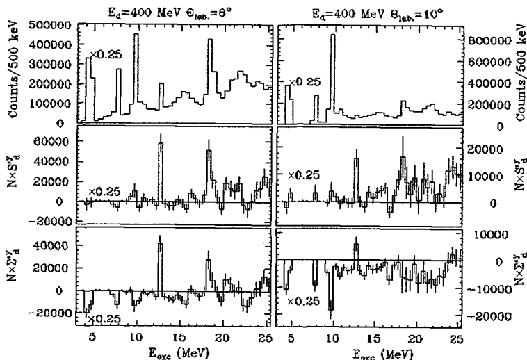
Fig. 2 - Inelastic ( d, d' ) spectrum measured at laboratory angles of 6^\circ and 10^\circ on ^{12}\text{C}
