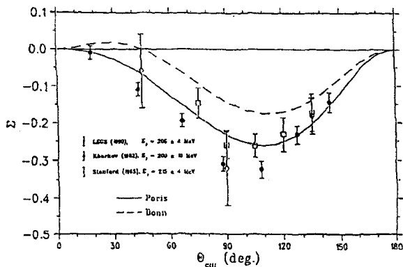
Fig. 4 - Photon polarization asymmetry as a function of c.m. proton angle at E_\gamma=206 Mev. Full circles-LEGS; open squares-Gorbunov et al./16/; open triangles-Liu /17/. Solid /11/ and dashed /12/ curves are theoretical calculations by Arenhövel using the Paris and Bonn potentials, respectively.
