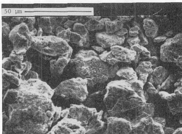
Fig. 3 : Amorphous powder after 30 hours milling with WC ball (residual O 2 atmosphere).
