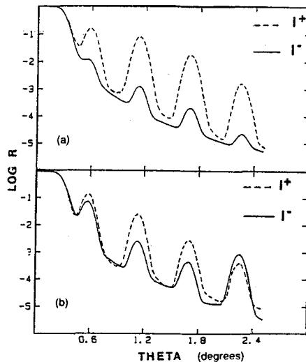
Fig.2: Calculated \theta/2\theta polarized neutron reflectivity (from scattering amplitude profiles of Fig.1) of Fe/Si multilayers with \lambda=2.36\text{\AA} :
