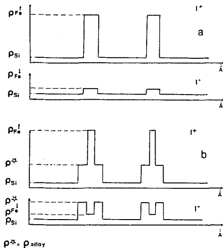
Fig.1: Schematic drawing of the neutron scattering amplitude density for a Fe/Si multilayer (50 bilayers - thickness of Fe=25Å and thickness of Si=95Å)
