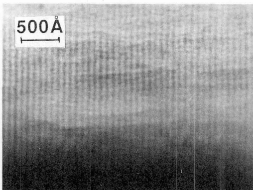
Fig.4: Cross-sectional electron micrograph of Si/Si:H/Si/Si:H multilayers
