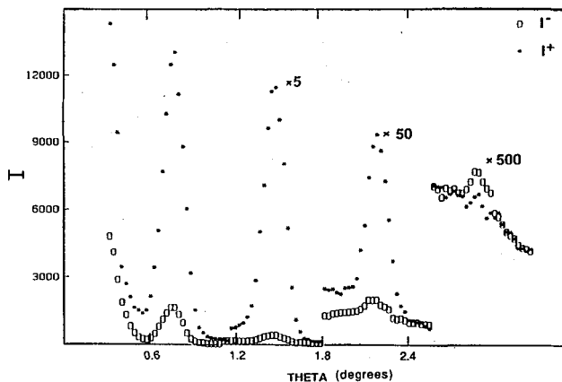
Fig.3: Experimental \theta/2\theta polarized neutron diffraction pattern from the Fe/Si multilayer ( \lambda=2.36\text{\AA} ). I^+ = intensity collected when the spins of the neutrons are parallel to the iron atomic moment. I^- = intensity collected in the antiparallel geometry.
