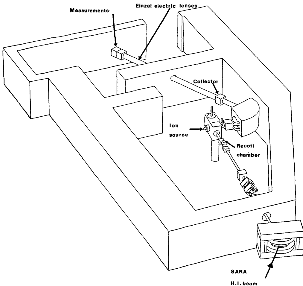
Figure 4 - The 120^\circ on-line isotope separator at SARA.
