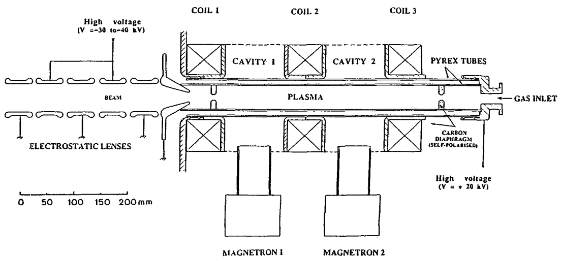
Figure 1 - Layout of the ECR ion-source system.
