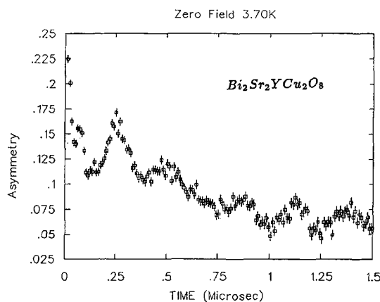
Fig. 4. - Asymmetry of muon decay signal observed in \mu\text{SR} measurement on a sintered pellet specimen of \text{Bi}_2\text{Sr}_2\text{YCu}_2\text{O}_8 at T = 3.7 K in zero field. The observed muon spin precession demonstrates that this material undergoes static magnetic ordering.
