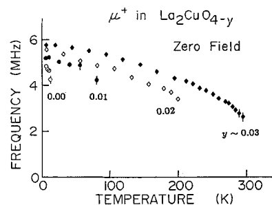
Fig. 1. - Muon spin precession frequency \nu_\mu observed in zero field on various sintered powder specimens of \text{La}_2\text{CuO}_{4-y} . The relative precision of y is \Delta y \leq 0.005 , while the absolute values of the stoichiometry of La, Cu, and O are subject to larger systematic errors (from Uemura et al. [4]).
