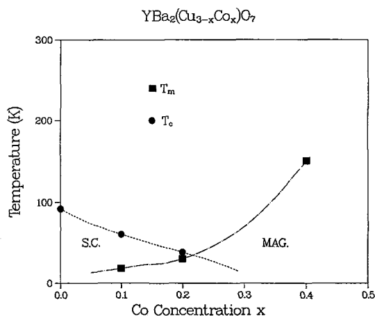
Fig. 3. - Phase diagram of the \text{YBa}_2(\text{Cu}_{3-x}\text{Co}_x)\text{O}_7 system determined by the \mu\text{SR} measurements (from Yu et al. [18]). S.C. denotes the superconducting state, and MAG. denotes the state with static magnetic order.
