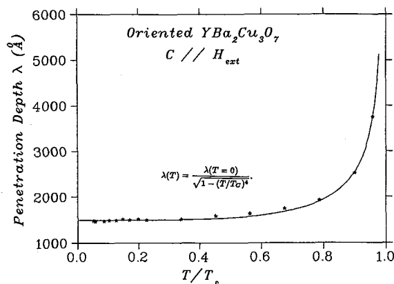
Fig. 6. - Temperature dependence of the magnetic field penetration depth \lambda_{\parallel} derived from the muon spin relaxation rate \sigma in a c -axis oriented sintered specimen of \text{YBa}_2\text{Cu}_3\text{O}_7 with the external field H_{\text{ext}} applied parallel to the c -axis. The solid lines represent fits of the data to the so-called empirical formula \lambda(T) = \lambda(T=0) / \sqrt{(1 - (T/T_c))^4} .
