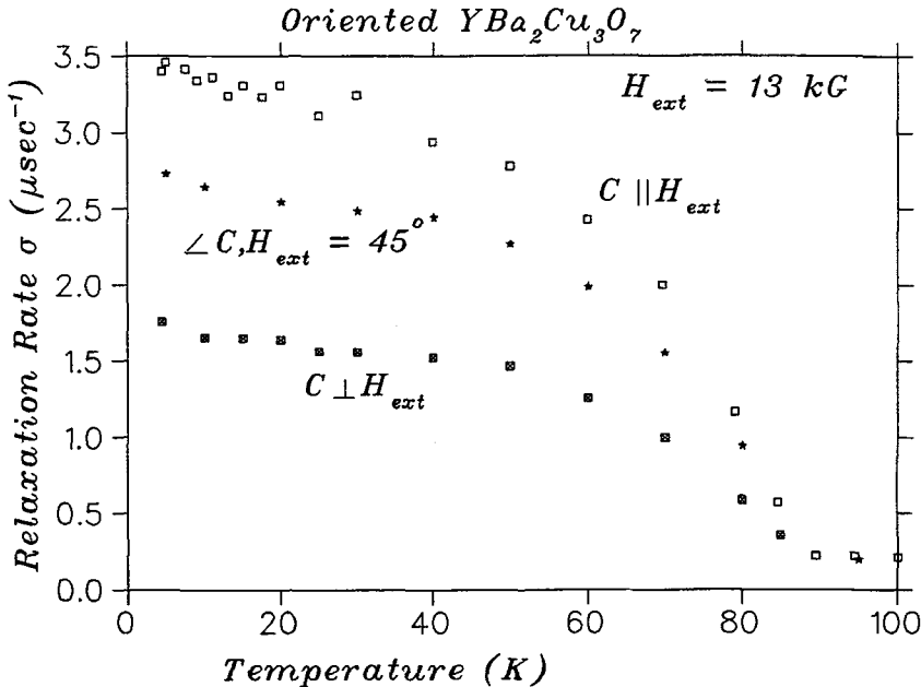
Fig. 5. - Muon spin relaxation rate \sigma observed in the TF- \mu SR measurements with H_{ext}=13 kG in the c -axis aligned pellet specimen of YBa 2 Cu 3 O 7 . The relaxation rate is largest when we applied H_{ext} parallel to the c -axis. This confirms the anisotropy of the penetration depth \lambda .
