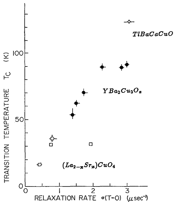
Fig. 7. - Superconducting transition temperatures T_c , as determined by \mu\text{SR} measurements, plotted against the values of the muon spin relaxation rate \sigma(T \rightarrow 0) for non-aligned pellet specimens of high- T_c superconductors ( \text{La}_{2-x}\text{Sr}_x ) \text{CuO}_4 , \text{YBa}_2\text{Cu}_3\text{O}_x , and \text{TlBaCaCuO} . A linear relation between T_c and \sigma(T \rightarrow 0) \propto 1/\lambda^2 \propto n_s/m^* is seen for the initial increase of \sigma(T \rightarrow 0) , while deviations from the linear line is noticed to take place at system-dependent values of \sigma .
