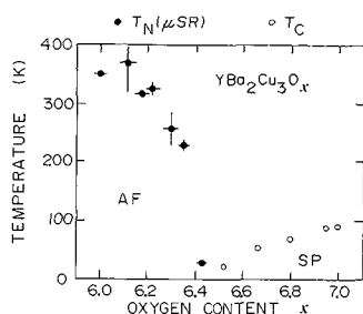
Fig. 2. - Phase diagram of \text{YBa}_2\text{Cu}_3\text{O}_x (specimens produced by rapid quenching) plotted against the oxygen concentration x . The closed circles stand for the Néel temperatures T_N determined by our \mu\text{SR} measurements (from Brewer et al. [3]), while open circles represent superconducting transition temperatures T_C determined by various methods. It is shown that the superconducting phase (SP) sets in around the oxygen concentration where the 3 dimensional magnetic order in the antiferromagnetic phase (AF) disappears.
