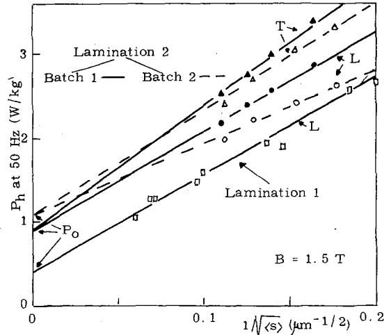
Fig. 2. - Hysteresis loss at 50 Hz and 1.5 T vs. 1/\sqrt{\langle s \rangle} , with \langle s \rangle average grain size. The experimental points have all been normalized to a given value of I_5 , through the linear equations displayed in figure 1. The background impurity contribution P_0 is given by intercepts of fitting lines given by equation (1) with the y -axis. L = longitudinal sheets, T = transverse sheets. Each line pertains to a different value of I_5 (in sequence 1.65, 1.70, 1.72, 1.78 T for lamination 2 and 1.77 T for lamination 1). The lines slope decreases with increasing I_5 .
