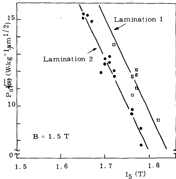
Fig. 1. - Experimental values of P_s = (P_h - P_0^*) \cdot \sqrt{\langle s \rangle} as a function of magnetization at 5 \times 10^3 A/m, I_5 , against best fitting lines A_0^* - k^* I_5 (see text and Eq. (1)).
