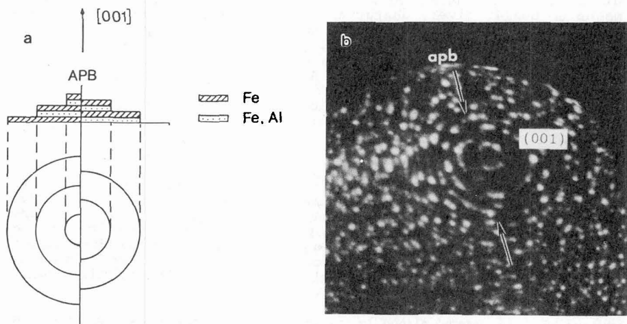
Fig. 2a - Schematic diagram of the FIM image of an anti-phase boundary on a [001] pole. Only the pure Fe planes are imaged since the mixed Fe and Al layers have preferentially evaporated. b - FIM image of an APB on a [001] pole from a DO_3 superlattice.
