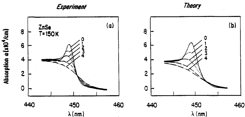
Fig. 1. (a) Experimental absorption spectra for a 0.55 \mu\text{m} ZnSe thin film at T = 150 K : 0) linear (no pump), 1) 2.5 kW/cm 2 , 2) 9 kW/cm 2 , 3) 23 kW/cm 2 , 4) 46.5 kW/cm 2 . (b) Calculated absorption spectra for different electron-hole pair densities : 0) 1 \times 10^{15} cm -3 , 1) 5 \times 10^{16} cm -3 , 2) 1 \times 10^{17} cm -3 , 3) 2 \times 10^{17} cm -3 , 4) 3 \times 10^{17} cm -3
