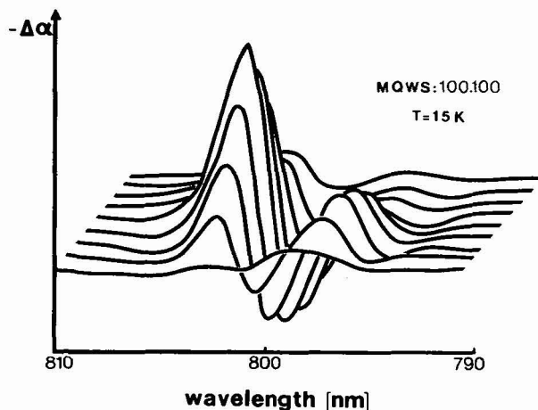
Figure 1 : Differential transmission spectra of a GaAs multiquantum-well-structure in the vicinity of the lowest (heavy-hole) exciton, recorded at 100 fs intervals, well thickness = 100 Å ; barrier thickness = 100 Å. Pump wavelength = 815 nm.
