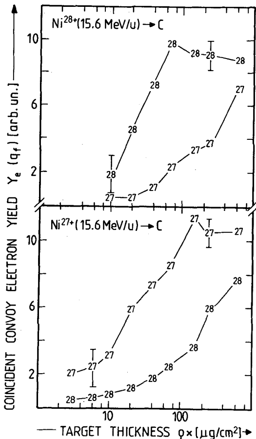
Fig. 2: Target thickness ( \rho x ) dependence of the convoy electron yield Y_e(q_f) for the incident projectile ions Ni^{28+} (top) and Ni^{27+} (bottom) E_p=15.6 MeV/u in coincidence with projectiles of the outgoing charge states q_f=28 and 27. The lines are drawn to guide the eye.
