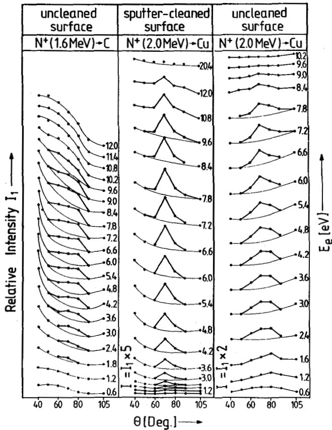
Fig.1: Angular distributions ( 40^\circ \leq \theta \leq 105^\circ ) of low energy secondary electrons at different electron energies 0.6 \text{ eV} \leq E_e \leq 20.4 \text{ eV} from a C-foil ( d=1000\text{\AA} ; left) and an uncleaned resp. sputter-cleaned Cu-foil ( d=1000\text{\AA} ; centre and right) bombarded with N^+ (see text). Note the different intensity scales!
