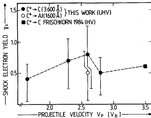
Fig.2: Number of shock electrons per incoming projectile \gamma_s as a function of the projectile velocity v_p .
