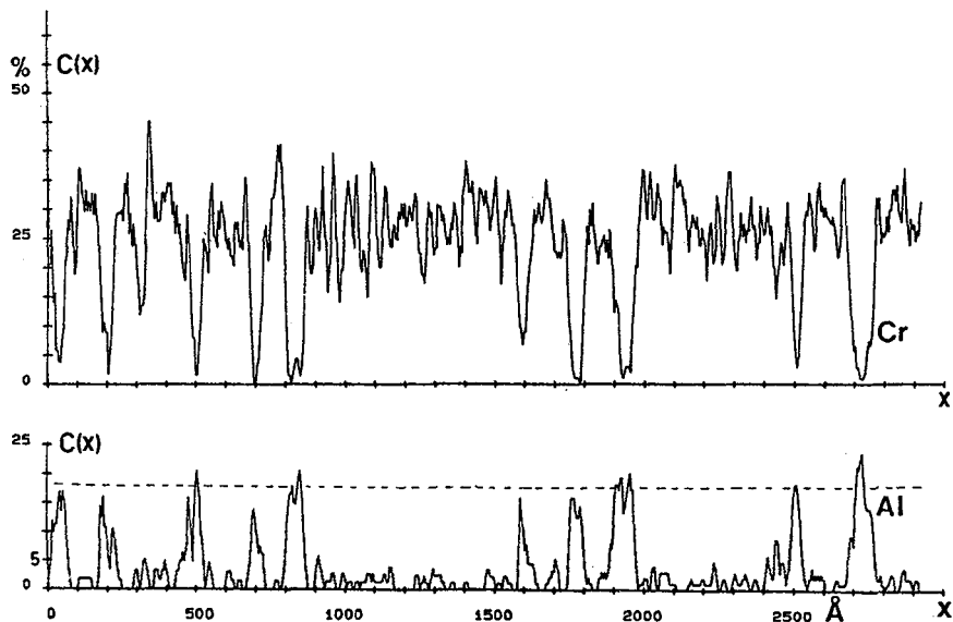
Figure 2 : Concentration profiles related to Al and Cr elements. \gamma' particles appear as Al rich zones.
