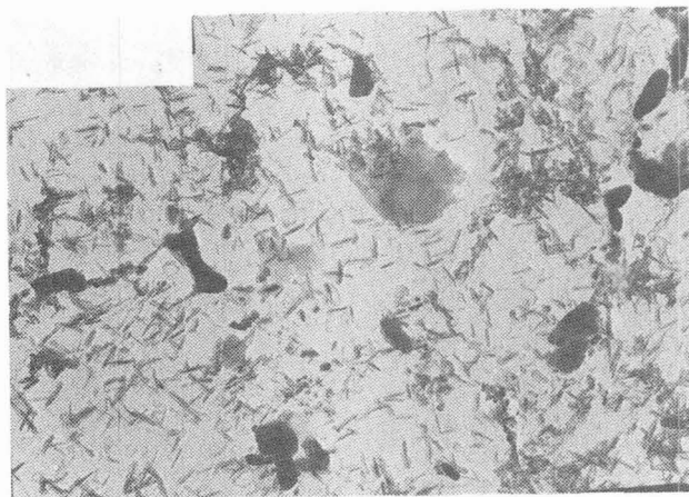
Fig. 6. Carbon extraction replica of the heat treated material. The needle-shaped particles are of M_2C -type and most of the dark areas are cementite. Some of the dark areas were found to be M_{23}C_6 particles by EDX-analysis.
