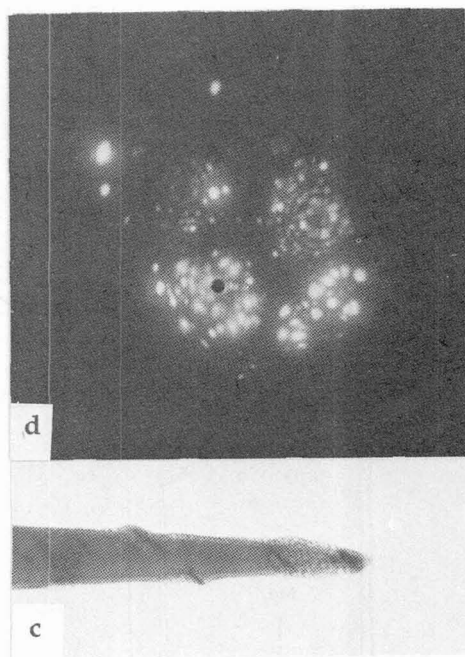
Fig. 7c. Bright field TEM micrograph of the specimen after heat treatment. M_2C precipitates can be seen.
