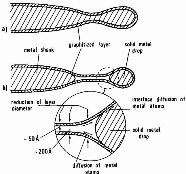
Fig. 9 - Explanation of the formation of a filiform neck.
