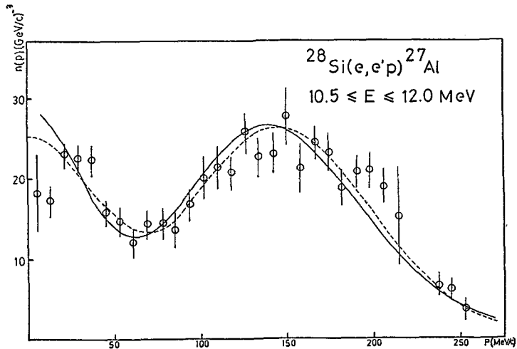
Fig. 2 - Comparison of deformed model result for \delta = 0.1 (---) to the experimental data and fit (7) .
