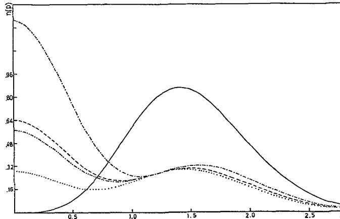
Fig. 1 - Momentum distribution for \delta = -0.2 (-.-), \delta = -0.1 (---), \delta = 0 (—), \delta = 0.1 (....), \delta = 0.2 (-.-.-)
