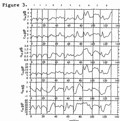
Figure 3. Capacitance and conductance values at 60 Hz, 12 kHz and 75 kHz for the top 6.6 m of the core. The first 3 sections numbered 1 are the same piece of ice. The ends of each section are shown with a vertical line. Each data set is represented by one position on the x axis.
