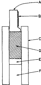
Figure 1. Density determination apparatus: A, right cylindrical glass plug; B, scale with .1 mm markings; C, thick - walled stainless steel tube; D, ice sample; E, hard soldered stainless steel plug; F, coupling space for mounting onto stem inside the high pressure cell.
