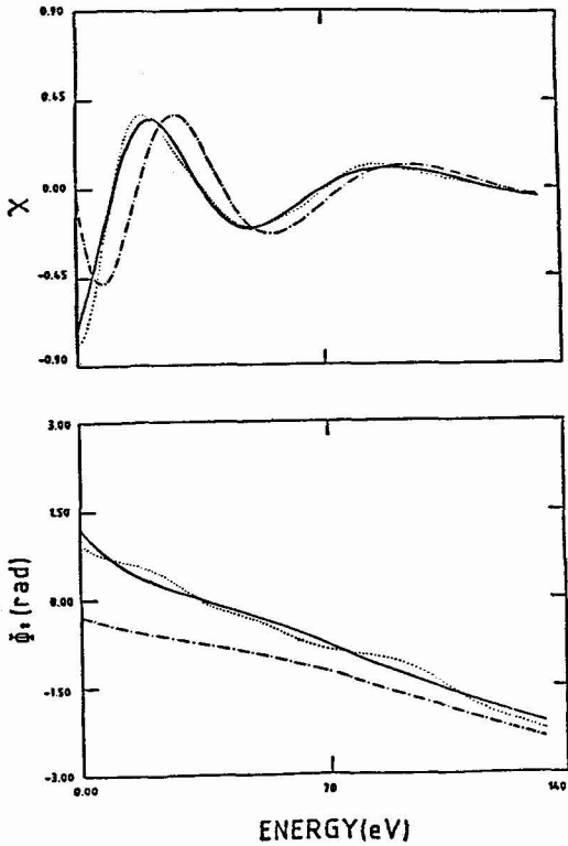
Figure 1 : Exact \chi_2^1 signal and phase function (dotted curves) for MnO_4 cluster, compared with S.W. approximation (Eq. 20) (full lines) and P.W. approximation (dot-dashed lines).
