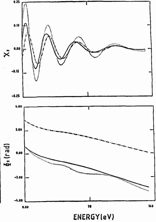
Figure 2 : Same as Fig. 1 for \chi_3^1 signal and phase function \phi_3 .
