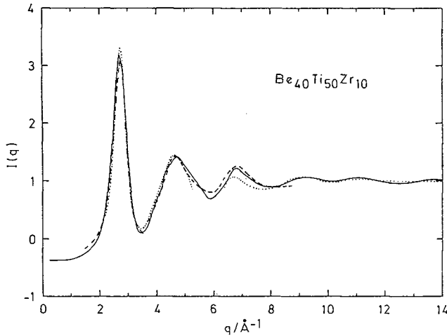
Fig. 3 - I(q) -data for \text{Be}_{40}\text{Ti}_{50}\text{Zr}_{10} as determined by the 2\theta -method (ADXD) and the \lambda -method (EDXD). The overlap of the different EDXD-data sets, taken at various fixed 2\theta -positions ( 6^\circ, 10^\circ, 20^\circ, 30^\circ ) is clearly seen.
