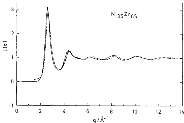
Fig. 4 - The same as Fig. 3 for \text{Ni}_{35}\text{Zr}_{65} .
