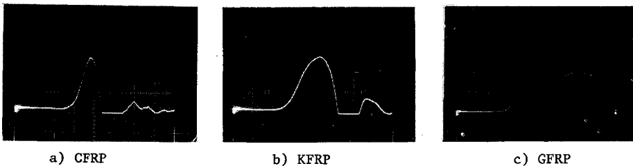
Fig.3 INERTIA-BAR STRAIN GAUGE SIGNALS FOR IMPACT TESTS (total sweep time - 100 \mu s)
