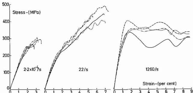
Fig.7 KFRP STRESS-STRAIN CURVES
