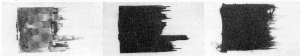
a) CFRP (reflected light: x3) b) CFRP (transmitted light: x3) c) KFRP (transmitted light: x3) Fig.8 FRACTURE APPEARANCE OF CFRP AND KFRP SPECIMENS
