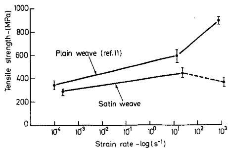
Fig.13 STRAIN-RATE DEPENDENCE OF TENSILE STRENGTH (woven GFRP specimens)
