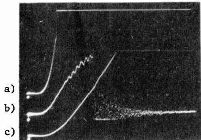
Fig.4 HYDRAULIC MACHINE TRACES CFRP Test: sweep time, 4ms a) Specimen strain b) Specimen load c) Crosshead displacement
