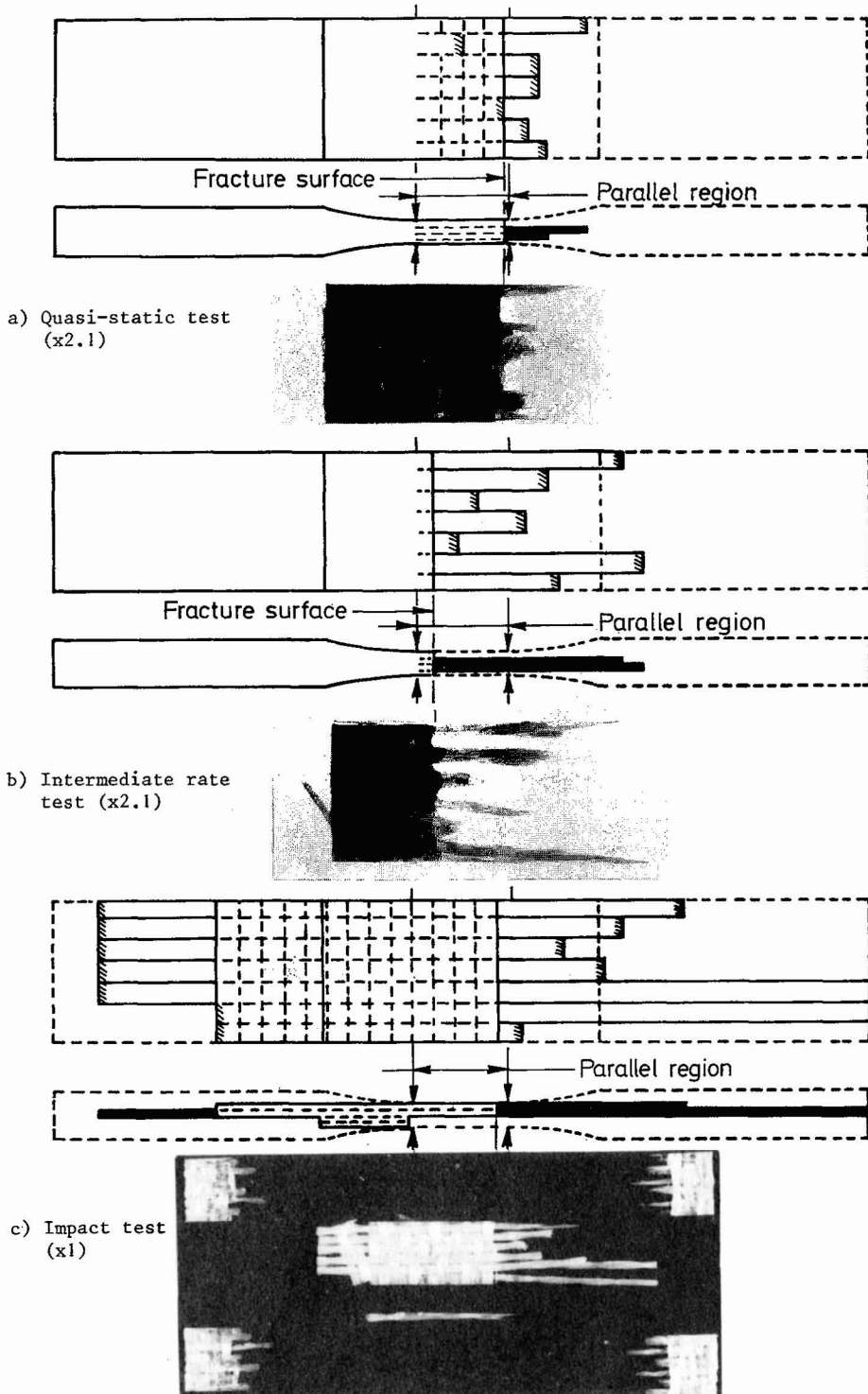
Fig.9 EFFECT OF STRAIN RATE ON FRACTURE APPEARANCE OF GFRP SPECIMENS
