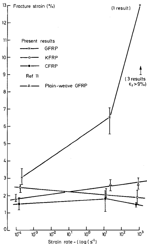
Fig.14 STRAIN-RATE DEPENDENCE OF FRACTURE STRAIN (woven GFRP specimens)
