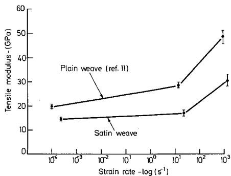
Fig.11 STRAIN-RATE DEPENDENCE OF TENSILE MODULUS (woven GFRP specimens)
