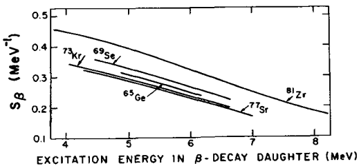
Fig. 12 Strength functions calculated according to the "gross theory" for the \beta -decay of T_{1/2} = 1/2 precursors.
