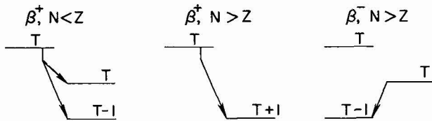
Fig. 1 Schematic illustration of the \beta -decays of various classes of nuclei showing the lowest-energy states with the indicated isospin.
