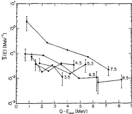
Fig. 8 Average \beta -strength function for 107 neutron-rich nuclei with 72 \leq A \leq 154 . Data are collected according to total Q_{\beta} (e.g. 7 \leq Q_{\beta} \leq 8 is labeled 7.5) and plotted against \beta energy. The ordinate of this figure, which is reproduced directly from ref /25/, must be multiplied by 0.62 to yield S_{\beta} as defined in eqn (5).
