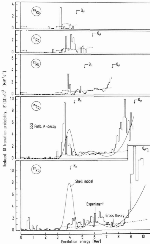
Fig. 15 Experimental \beta -strength functions of odd-mass rubidium isotopes plotted as a function of excitation energy in their daughters and taken from ref /30/. The quantity B^+(GT) is essentially equivalent to S_\beta as defined in eqn (5). The Q_\beta and neutron separation energy, B_n , are noted. For comparison, calculated strength functions are shown from the "gross theory" /28/ and a shell-model RPA approach /31/.
