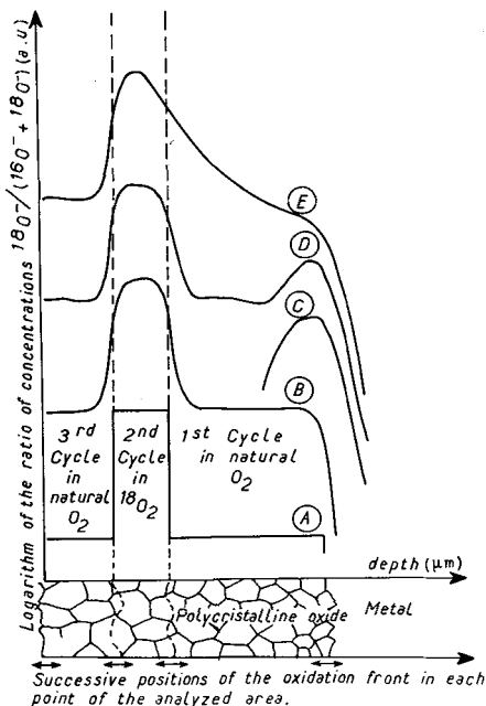
Fig. 1 - SIMS profiles of the depth distribution of an 18 O tracer in oxide films (5.5 keV Ar + bombardment under residual vacuum) :
