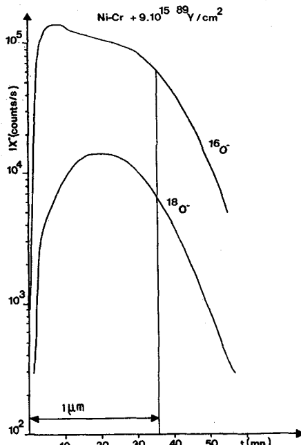
Fig. 4 - SIMS profile of the depth distribution of an 18 O tracer in the Cr 2 O 3 film formed at 800°C on 63 Ni/ 37 Cr doped with 9 \cdot 10^{15} Y/cm 2 of 100 keV. The Y concentration in the film is about 300 ppm (3).
