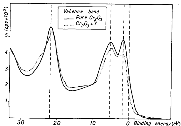
Fig. 5 - Part of the XPS spectrum recorded on \text{Cr}_2\text{O}_3 doped with 10^{16} \gamma/\text{cm}^2 of E = 100 \text{ keV} , after sputtering 30 nm. The conditions of analysis are the same as for Fig. 3. The differences in the intensities of O2s peaks (at 22 eV), O2p peak (at 5.3 eV) is due to a difference in the analysed areas. Their slight shift of 0.1 eV is due to a difference in charge accumulation. The peak at 2.2 eV is relative to uncoupled Cr3d electrons.
