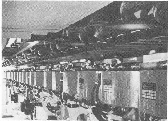
Figure 1: Supporting Magnets on Test Carrier TRO6 (Emsland Transrapid Test Facility)
