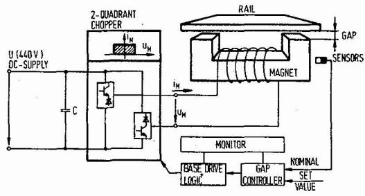
Figure 2: Magnet Control Circuit
