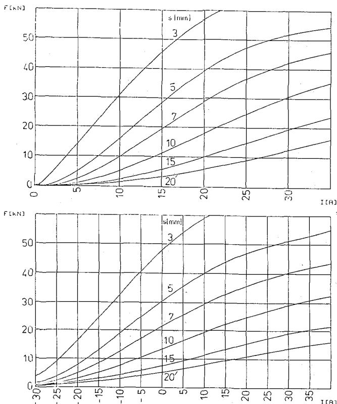
Figure 5: Stationary Characteristic Curves a) E-Magnet b) P-Magnet
