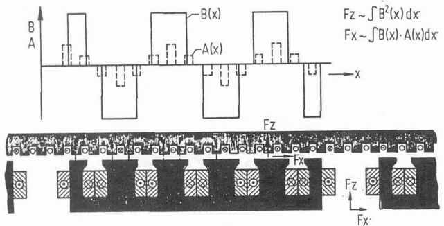
Figure 3: Principle of the Synchronous, Long-stator Motor with Iron Core
