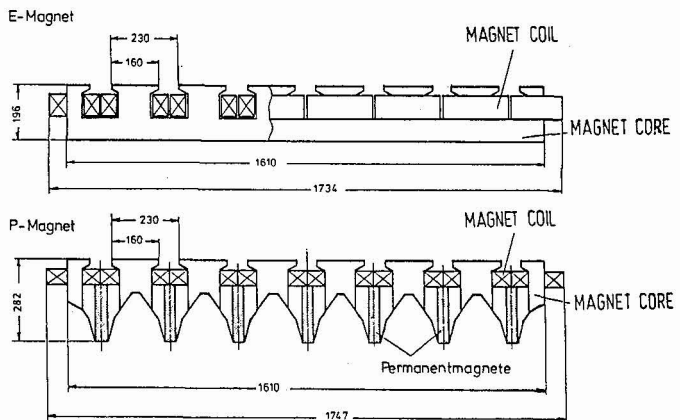
Figure 4: Electromagnet and Permanentmagnet
