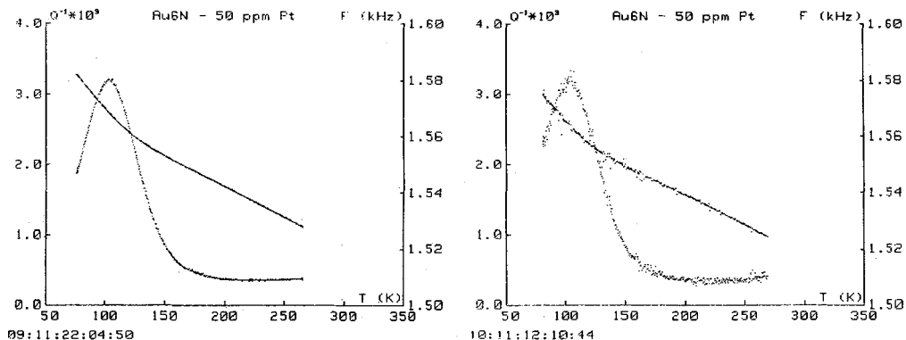
Fig. 4 : Results obtained in kilocycle range apparatus : Bordoni peak in Au 6N -50 ppm Pt at different strain amplitudes : a) 8 \cdot 10^{-7} b) 6 \cdot 10^{-8}
