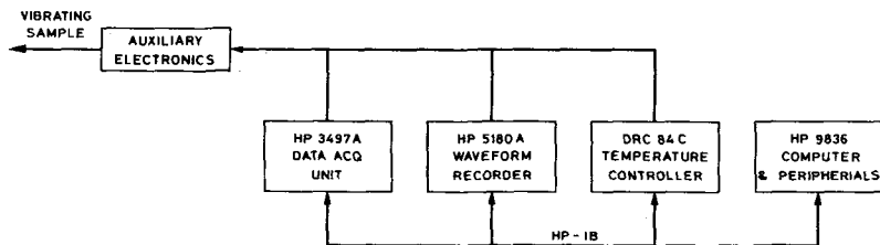
Fig. 3 : Block diagram of electronic part for kilocycle range apparatus.
