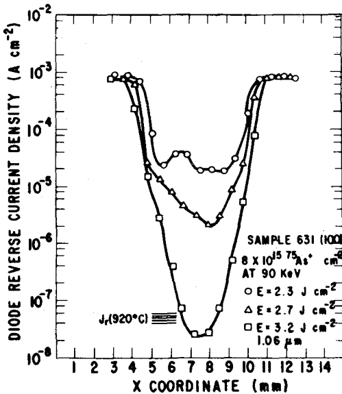
Fig. 5 (a) - Diode leakage current density for samples implanted at 90 keV with an As fluence of 8 \times 10^{15} \text{ cm}^{-2} . The laser annealing energy density was 2.3 \text{ J cm}^{-2} (○), 2.7 \text{ J cm}^{-2} (△), and 3.2 \text{ J cm}^{-2} (□), respectively. The data for a thermally-annealed diode are shown for comparison ( T = 920^\circ \text{ C} ). /11/.
