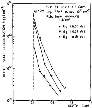
Fig. 4 - Depth profile of the three defects after 1 J/cm 2 ruby laser annealing. The limit of measurements at zero bias voltage is given by the dashed line. /7/.
