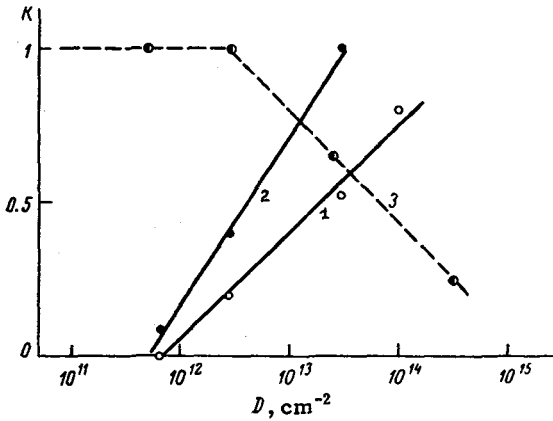
Fig. 8 - Dependence of the impurity utilization coefficient on the phosphorus ion dose after laser (1, 2) and thermal (3) annealing. Laser pulse energy ( \text{J}/\text{cm}^2 ) : 1) 1.6; 2) 2.5. Thermal annealing at 700° C for 15 min. /25/.
