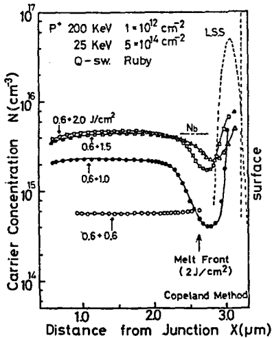
Fig. 7 - Carrier profiles of the double irradiated samples /18/
