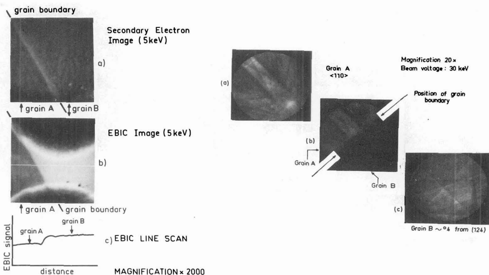
Fig. 6 : Difference in current collection between two adjacent grains seen by EBIC line scan.
