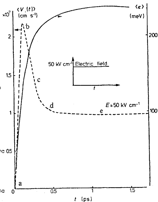
Figure 1. Transient drift velocity ( v ) and average energy ( \epsilon ) resulting from a time step of the electric field (n-Si, E \parallel \langle 111 \rangle , T = 293\text{ K} ).
