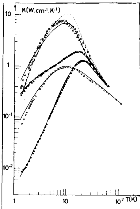
Fig.1 - Thermal conductivity versus the temperature for symbols see. Table 1
