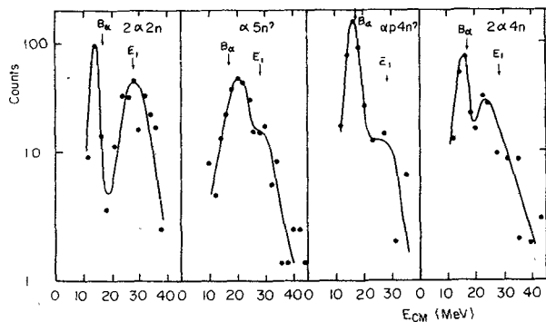
Fig. 3 : The same as fig. 1.a coincident with different Ge lines.
