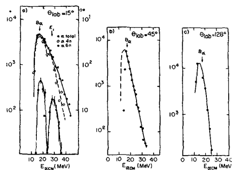
Fig. 2 : Center of mass \alpha particles spectra at 15° and 45° for 116 Sn + 16 O(a-b) and at 128° for 92 Zr + 40 Ar(c). On part a are also indicated the \alpha particles spectra coincident with \gamma lines identifying the \alpha 4n and \alpha 6n channels. B_\alpha indicates the coulomb barrier for an \alpha particle in the compound nucleus. E_\alpha indicates the energy of an \alpha particle having the same velocity as the incoming projectile. The low energy part of the 45° spectrum (1-b) is cut by a 120 \mu Al absorber.
