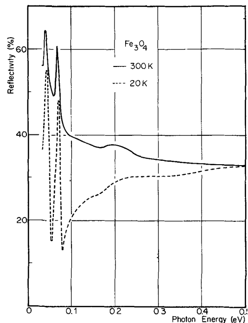
Fig.1 : Reflectivity of magnetite at 300 K (solid line) and at 20 K (broken line).
