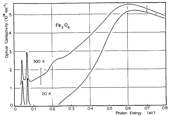
Fig.3 : Optical conductivity of magnetite at 300 K and 20 K from the Kramers-Kronig analysis.
