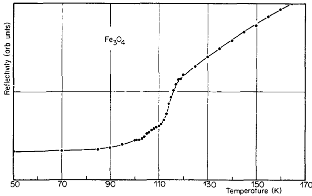
Fig. 2 : Temperature dependence of the reflectivity of magnetite at a photon energy of 0.0558 eV ( 450 \text{ cm}^{-1} ) near the Verwey-transition temperature.
