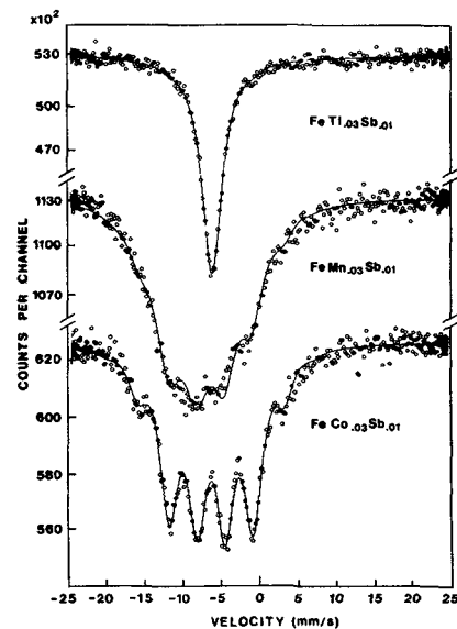
Fig. 1 : ^{121}\text{Sb} Mössbauer spectra of \text{FeSb}_{0.01}\text{M}_{0.03} alloys annealed at 500°C. The \text{FeSb}_{0.01}\text{Co}_{0.03} spectrum is typical for solute Sb atoms in \underline{\text{Fe}}\text{SbM} solid solution.
