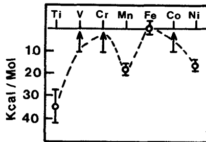
Fig. 2 : Orders of magnitude of the SbM interaction energies in dilute \text{Fe-Sb-M} alloys versus M.
