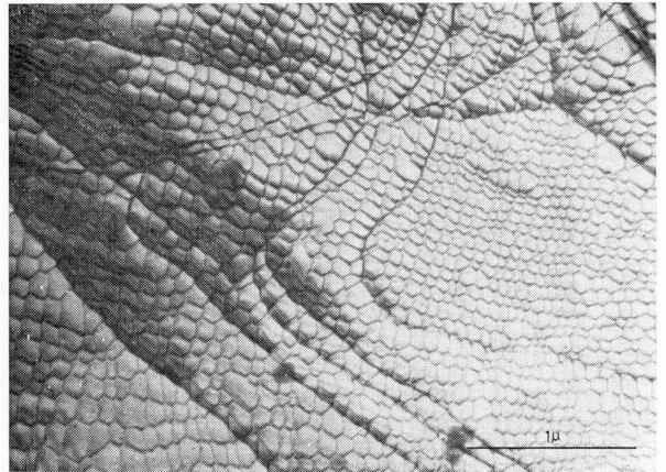
FIG. 10. — Hexagonal network of perfect dislocations in Bi_2Te_3 .
