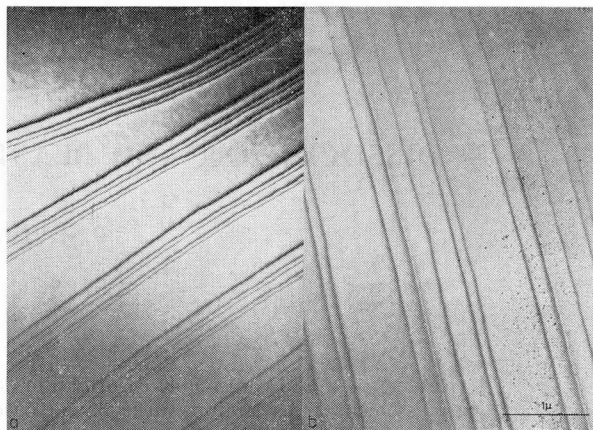
FIG. 3. — Dislocations in (a) \text{CrBr}_3 and in (b) \text{CrCl}_3 . The ribbons are clearly made of six partials, which is the most common dissociation type in these structures, although a dissociation in four partials is also possible.
