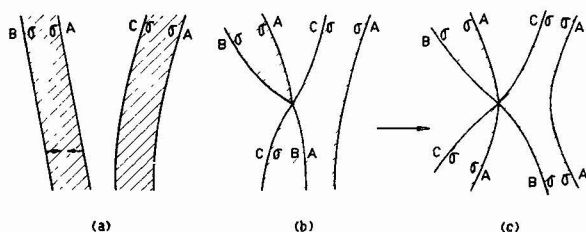
FIG. 6. — Proposed mechanism effectively occurring for the intersection of two extended dislocations BA and CA. The intersection is only possible after recombination of one of the extended ribbons. Here the recombination of the ribbon BA is presented in (b).
