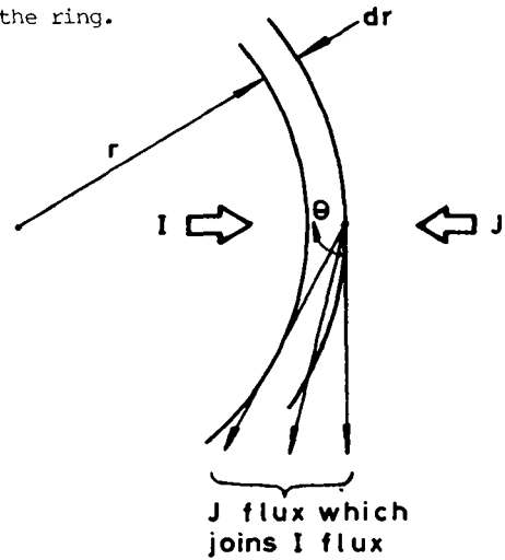
Fig. 2. Sketch showing radiation fluxes
