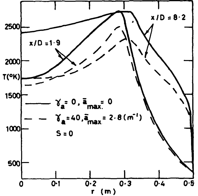
Fig. 4: Temperature profiles
