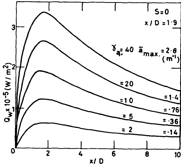
Fig. 3. Distribution of wall heat flux
