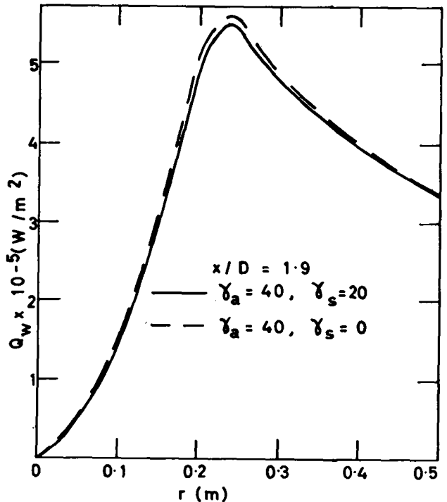
Fig. 6: Effect of scattering
