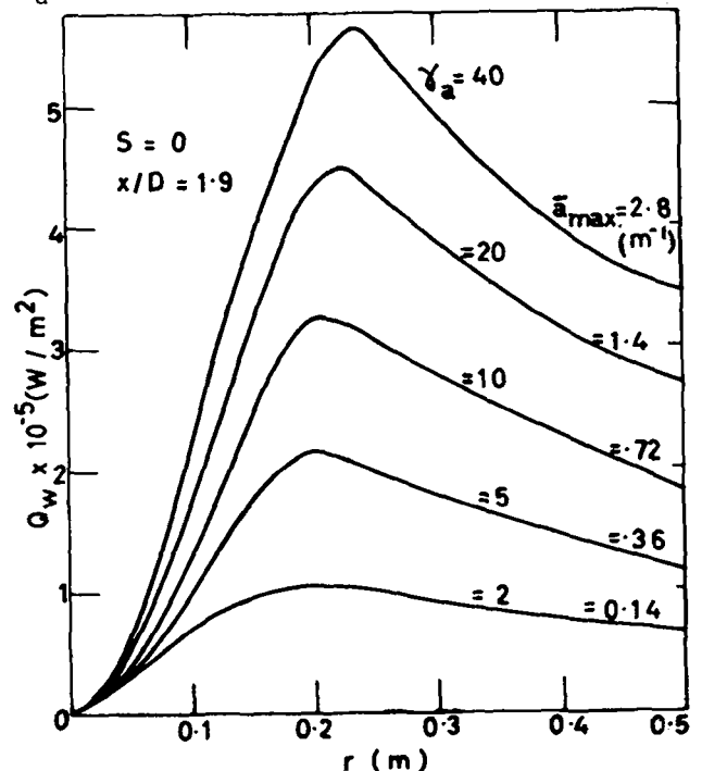
Fig. 5 Heat-flux profiles
