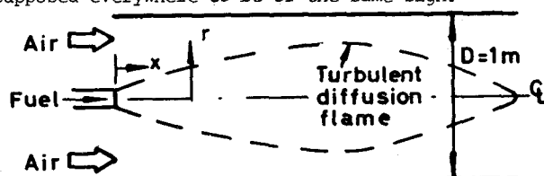
Fig. 1 Geometry and flow conditions of the problem solved
