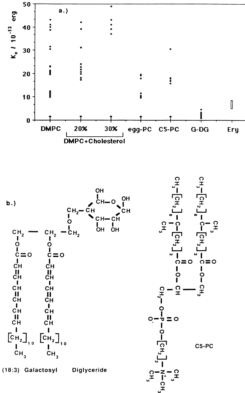
Fig. 7. — a) Summary of bending elastic moduli, K_c , of vesicles of various synthetic and natural lipids and of DMPC-cholesterol mixtures. On the right side the value of red blood cell membrane is shown. The lipid C5-PC is a phosphatidylcholine (PC) with a branched chain. G-DG (= galactosyldiglyceride) is a plant cell lipid with a high content of C = C -double bonds. Each point was obtained by evaluation of one single vesicle. Note that the values for DMPC, DMPC + 20 % cholesterol egg PC and C5-PC form well separated groups. The differences between the average values of K_c of adjacent groups are equal to the lowest value of K_c . Thus each group corresponds to vesicles with the same number of bilayers per cell. The lowest average K_c -values are summarized in table II. b) Structure of lipid C5-PC and G-DG.
